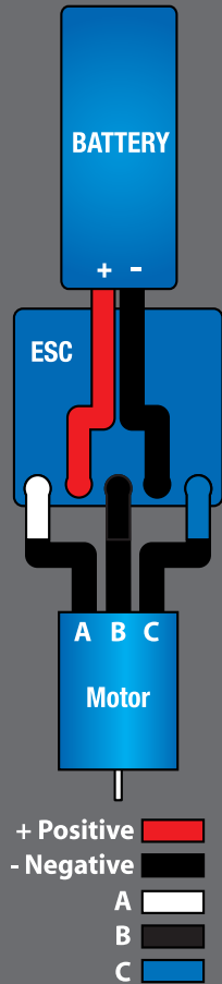
VX3 Wiring Diagram
